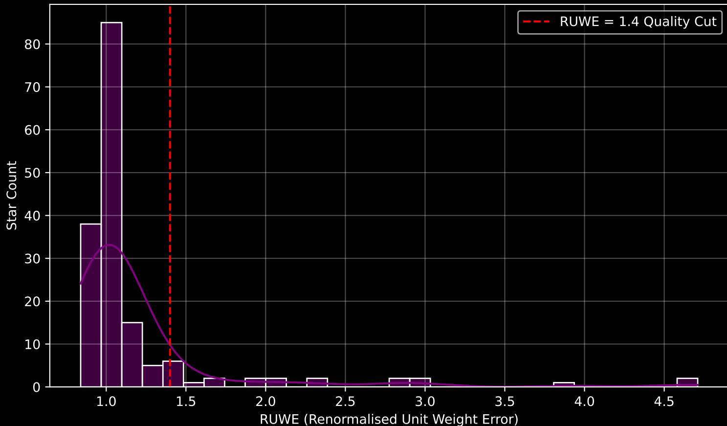
GAPOGEE DR17 Field [057+41_MGA] RUWE Distribution (n= 165)
