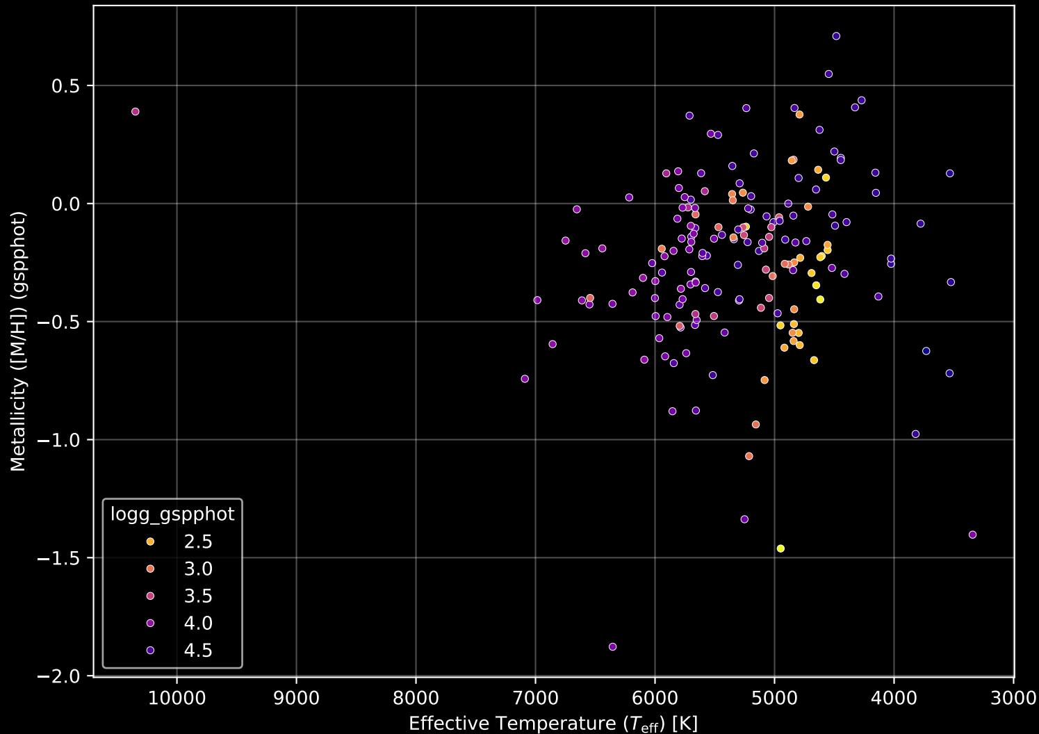
APOGEE DR17 Field: [057+41_MGA] Stellar Population Parameters (n= 176)
