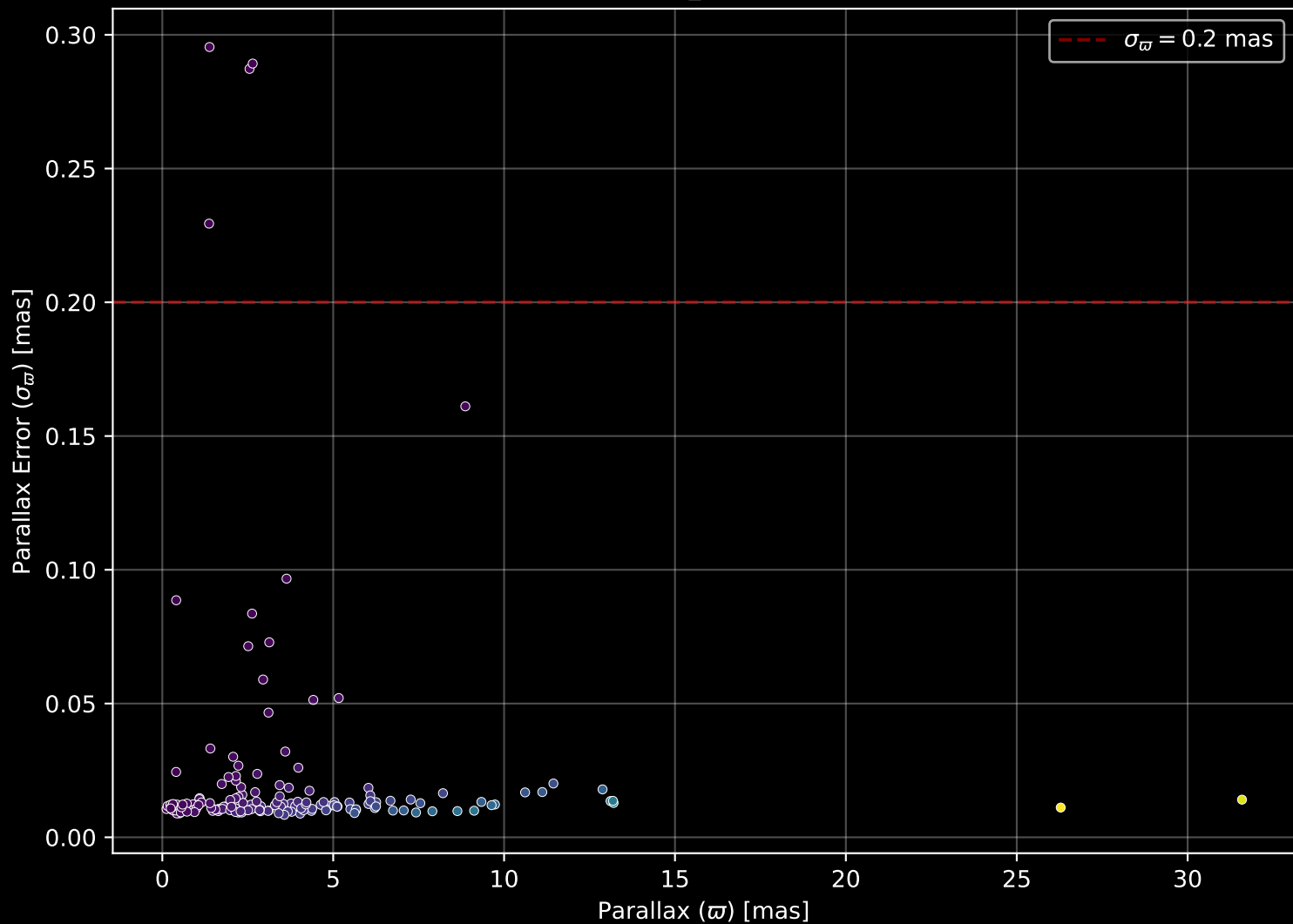
APOGEE DR17 Field: [057+41_MGA] Parallax Quality (n= 176)
