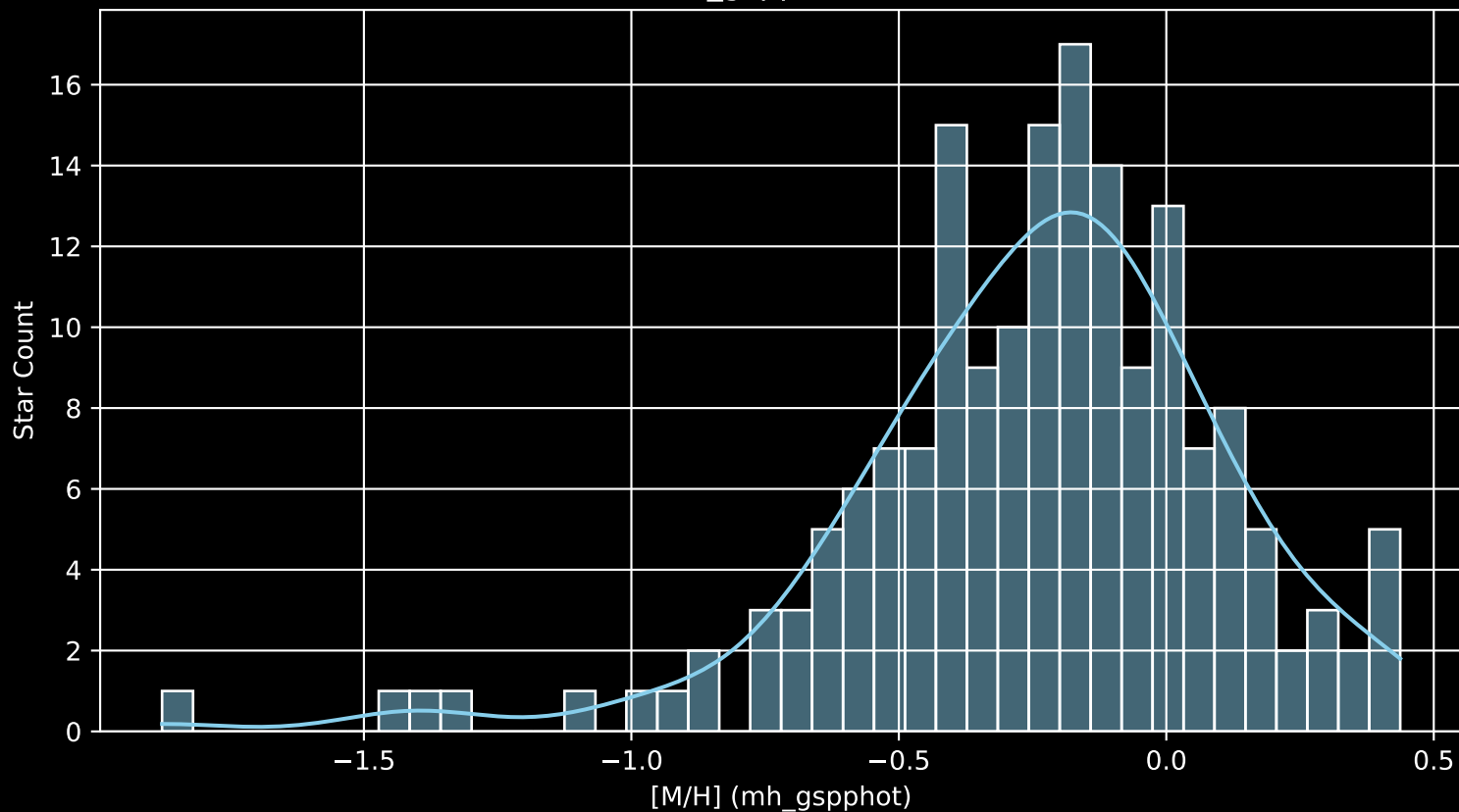
APOGEE DR17 Field: [057+41_MGA [M/H] (mh_gspphot) (n= 174)
