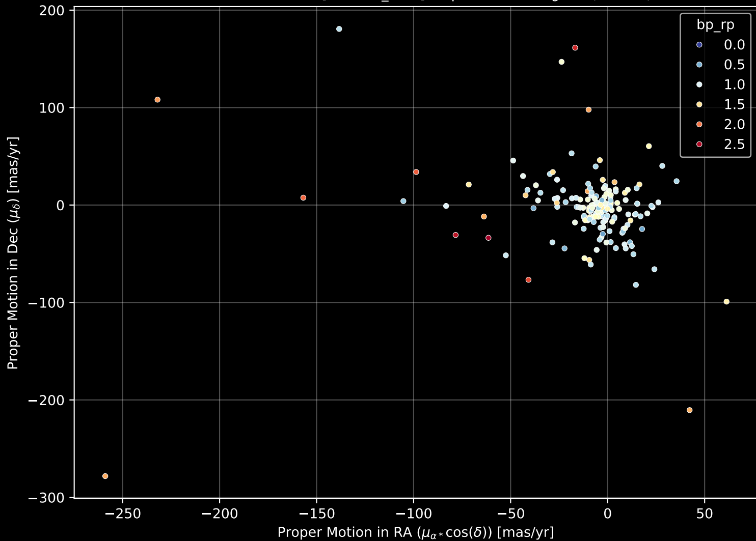
APOGEE DR17 Field: [057+41_MGA] Proper Motion Diagram (n= 176)
