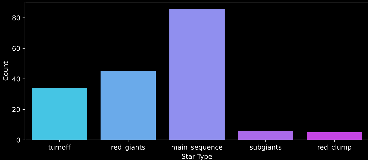
APOGEE DR17 Field: [057+41_MGA] Count plot of Star Type
